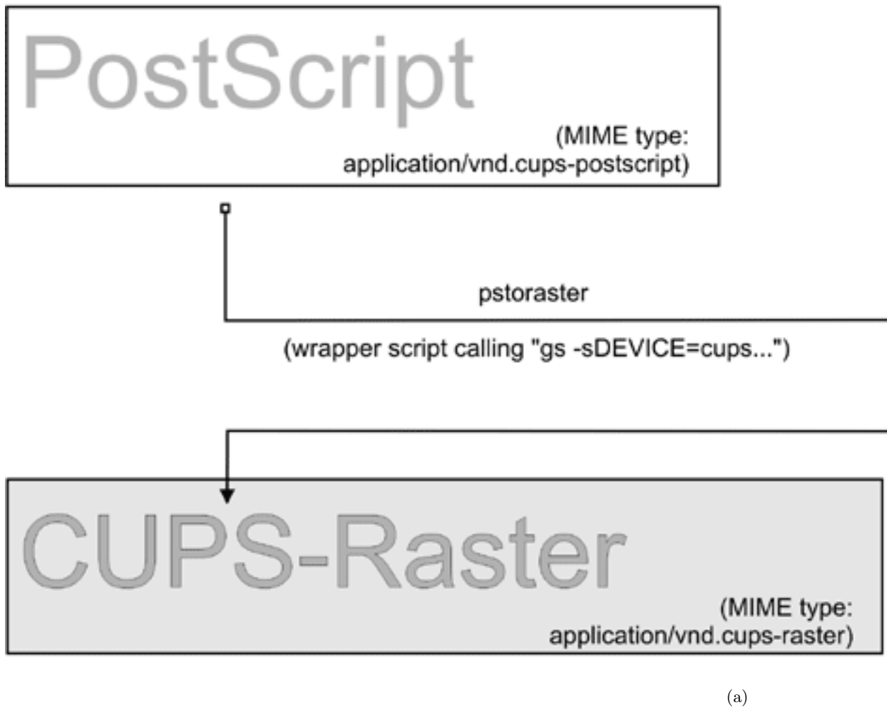
Figure 19.7: CUPS-raster production using Ghostscript
